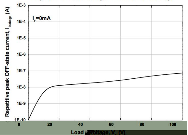
Figure 6. Off state leakage Current vs Load voltage
