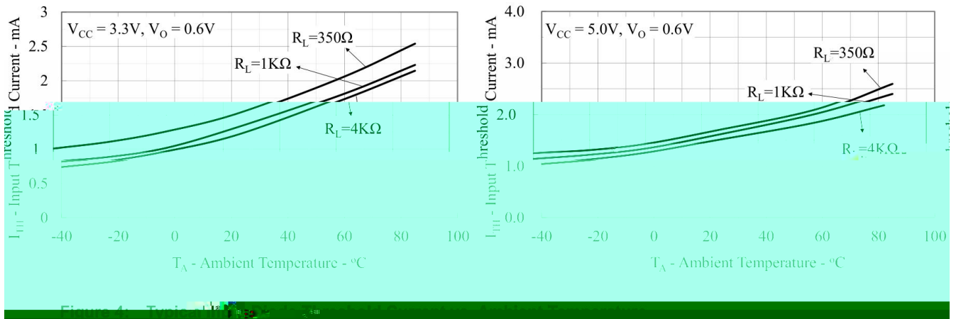
Figure 4: Typical Input Threshold Current vs. Ambient Temperature
