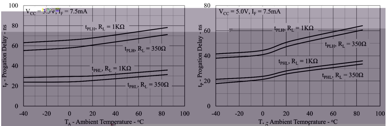
Figure 7: Typical Propagation Delay vs. Ambient Temperature
